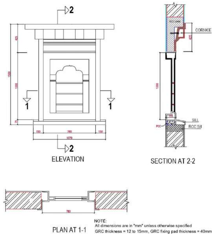
Fig 5.11.9 GRC Window 1 Bay 780mmX1385mm (Full set)
