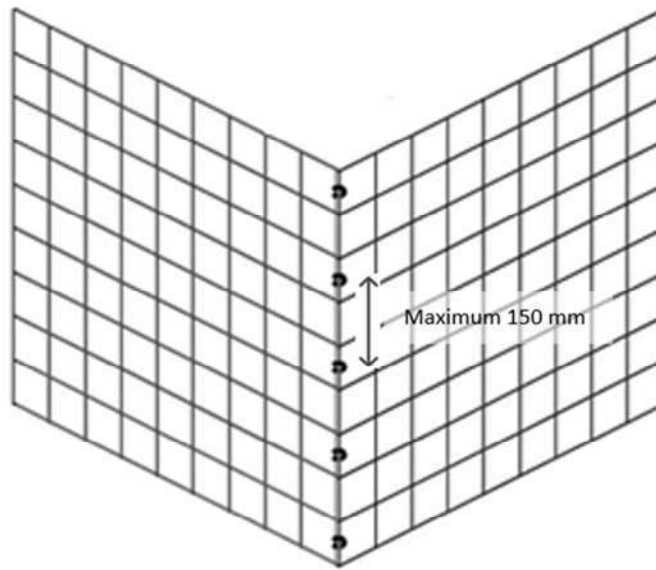
Figure 10 Ring type fasteners
