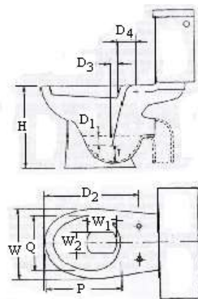
b. WASHDOWN WATER CLOSET FOR CLOSE COUPLED SUITE, P OR S TRAP
