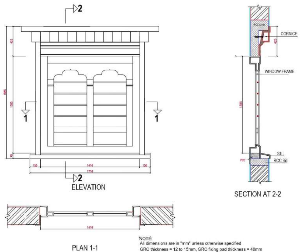
Fig 5.11.10 GRC Window 2 Bay 1416mmX1385mm (Full set)
