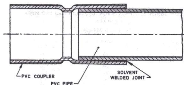
Figure 5.17.1 PVC solvent welded joint
