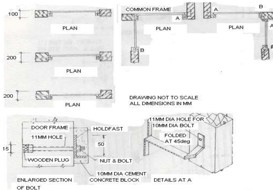
Fig 5.11.7 Arrangement of holdfast
