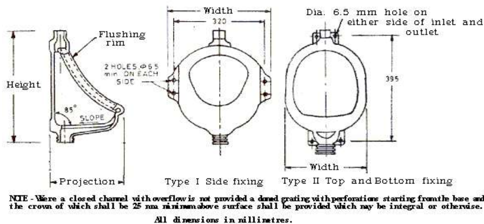
Figure 3.17 (c) BOWL PATTERN URINAL (FLAT BACK) WITH FLUSHING RIM
