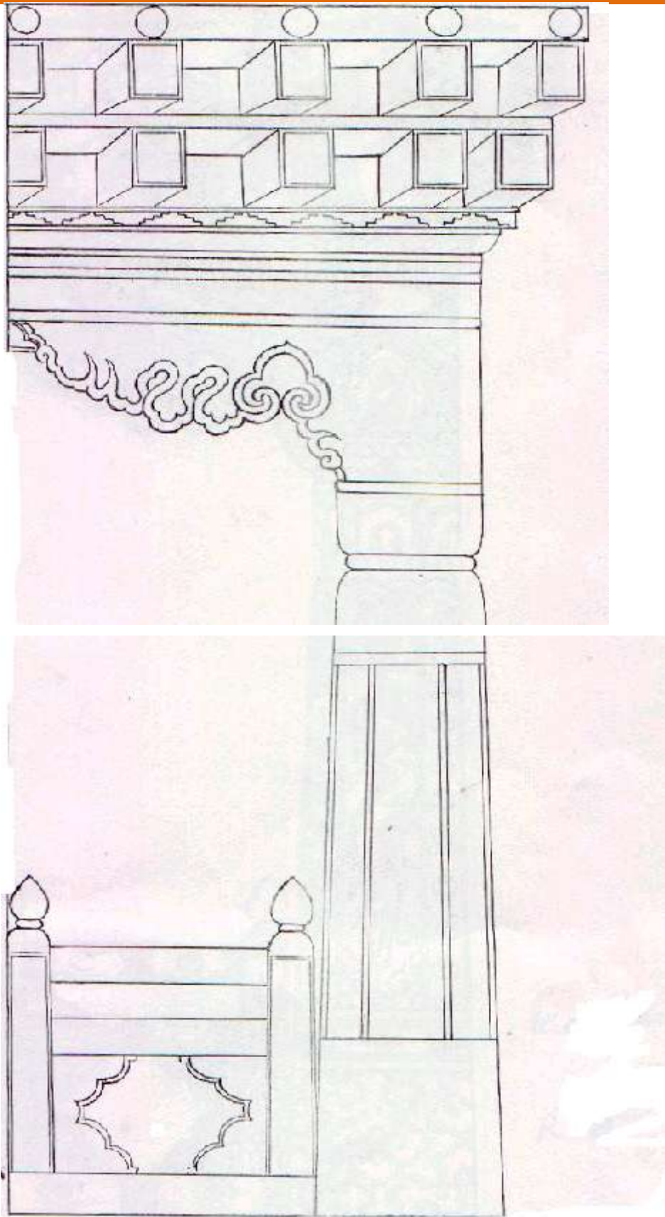
Figure 5.19.13 Kachen (Yutshon)
