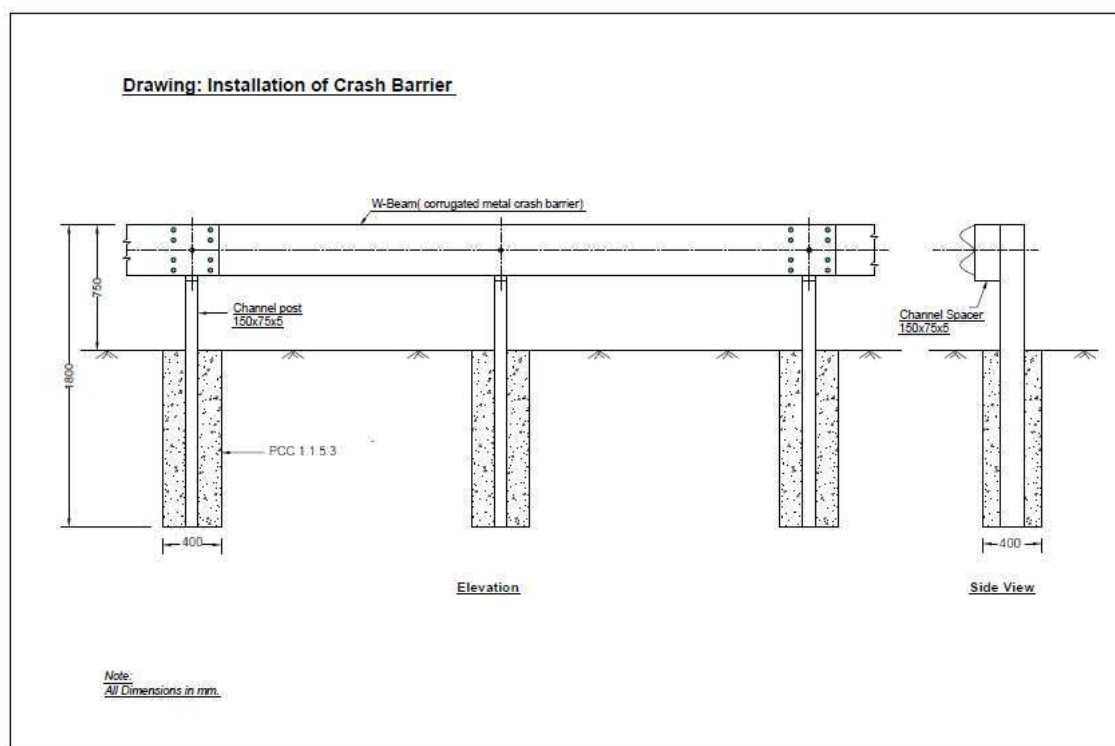
Figure 5.21.4 Crash Barrier
