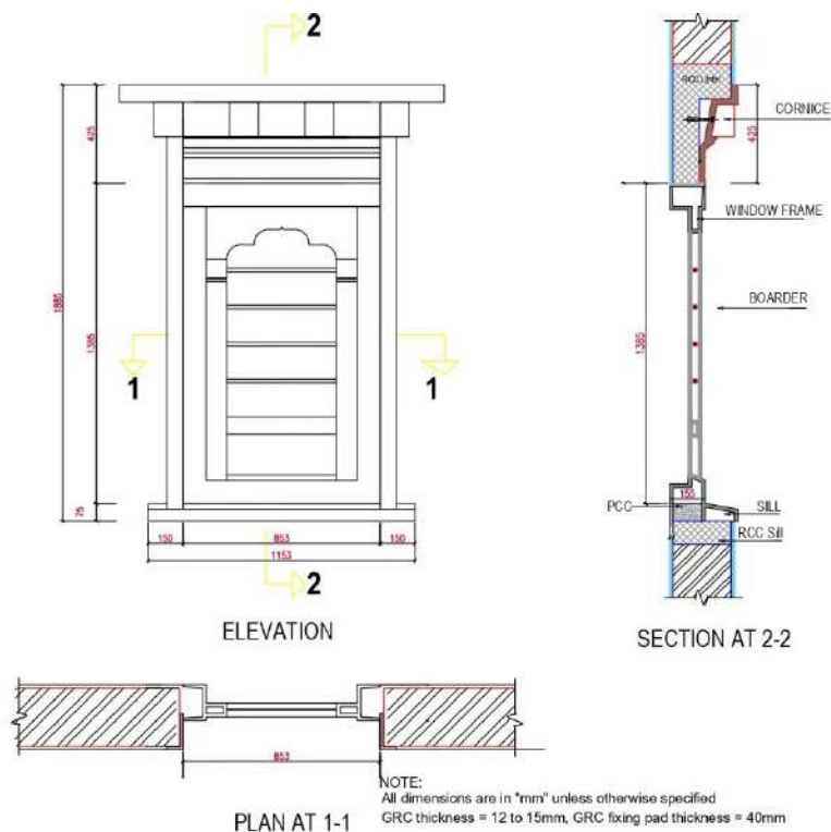
Fig 5.11.8 GRC Window 1 Bay 853mmX1385mm (Full set)
