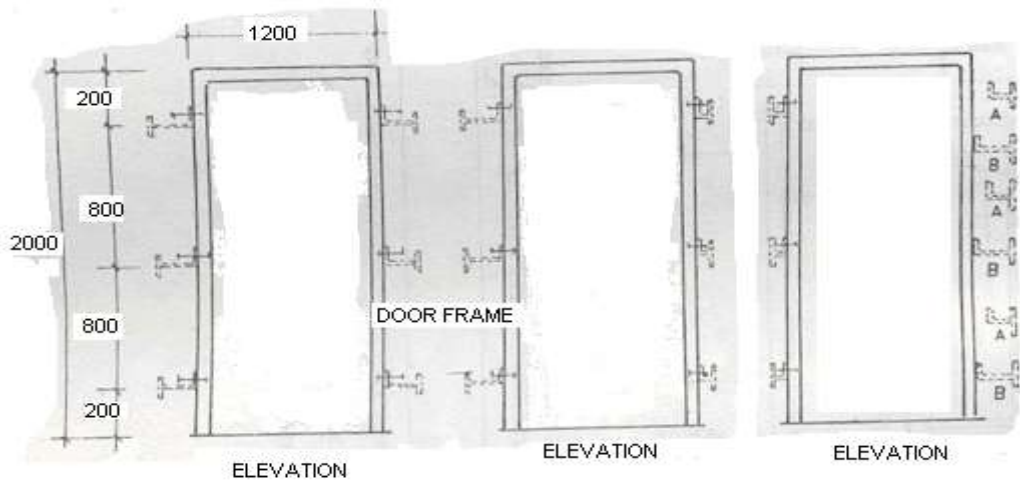
ARRANGEMENTS OF HOLDFAST
