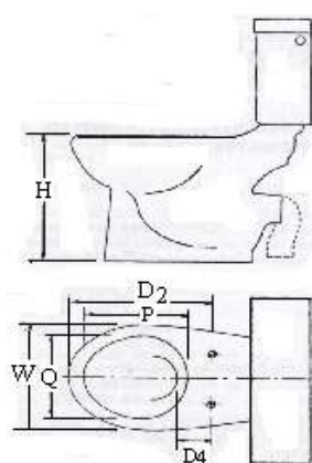
a. SYPHONIC WATER CLOSET - SINGLE OR DOUBLE TRAP PATTERN
