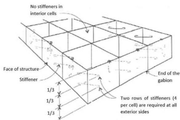
Figure 12 corner stiffener details
