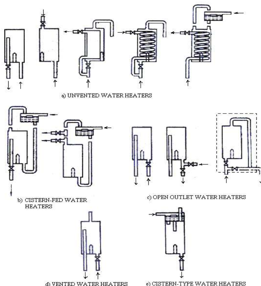
Figure 3.22 SCHEMATIC REPRESENTATION OF STORAGE WATER HEATERS
