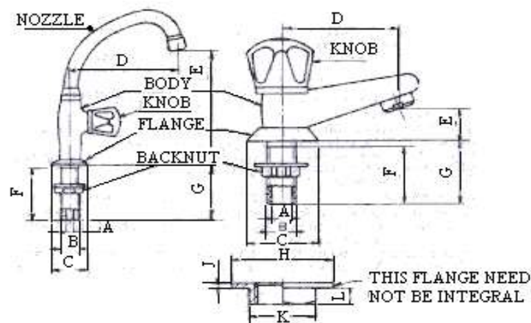
Figure 3.10 BODIES FOR PILLAR TAPS (TYPICAL DETAILS)
