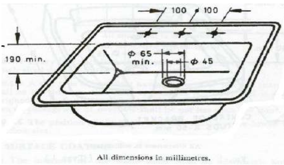
a. FLAT-BACK WASH BASIN (TYPE II)
