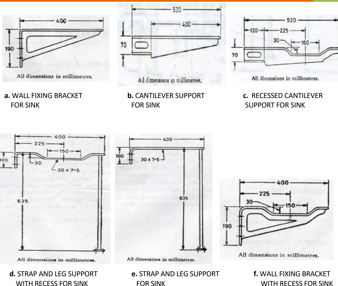
Figure 3.20 R.S OR C.I BRACKETS AND SUPPORTS
