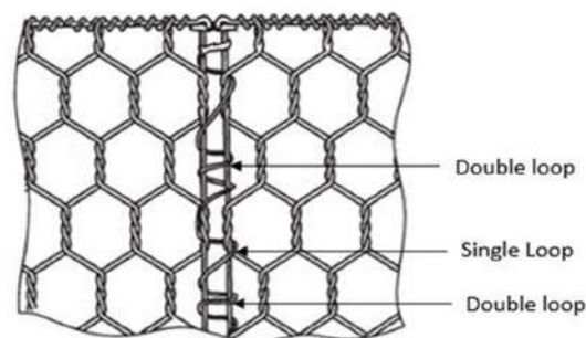
Figure 4 Rings for joining adjacent panels instead or with lacing wire
