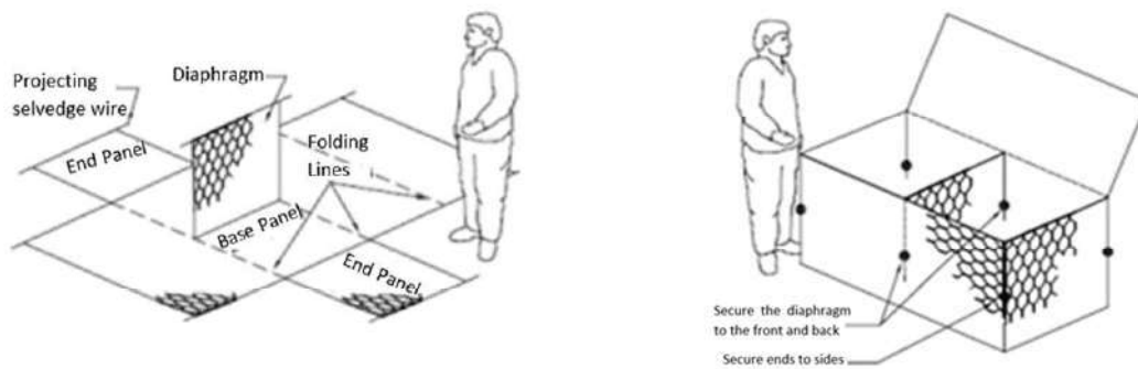
Figure 1 (a) and (b) Gabion installation
