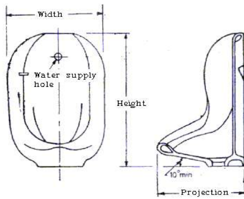
Figure 3.17 (a) BOWL URINAL FLAT BACK (WITHOUT FLUSHING RIM)
