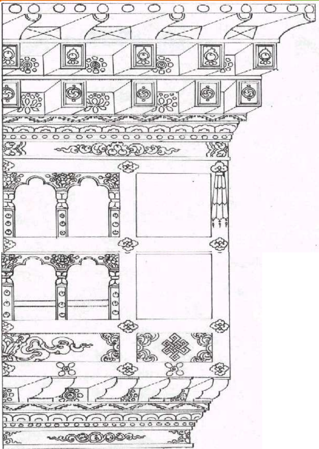
Figure 5.19.4 Rabsey (Dring)
