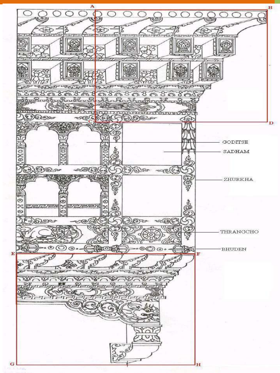
Figure 5.19.1 Rabsey (Rab)
