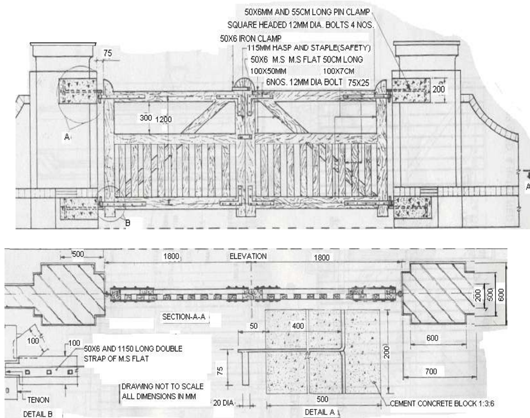
Figure 5.11.1 Details of compound gate
