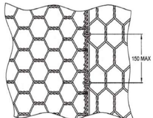
Figure 3 Lacing Wire for tying adjacent panels in single and double loop fashion
