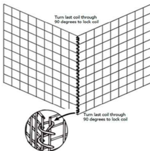
Figure 9 Spiral fastener
