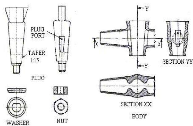
Figure 3.9 PLUG COCK AND COMPONENT PARTS
