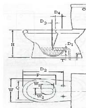
d. HORIZONTAL OUTLET WC FOR CLOSE COUPLED SUITE
