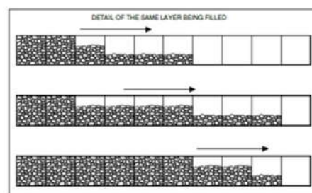
Figure 6 Filling pattern of gabion boxes
