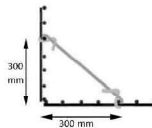
Figure 13 Layout of exterior corner stiffeners. Should be properly crimped
