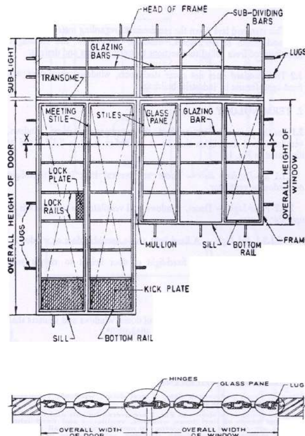
Figure 3.1 TERMINOLOGY FOR STEEL DOORS, WINDOWS AND SUB-LIGHT
