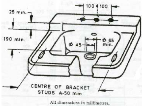
a. FLAT-BACK WASH BASIN (TYPE II)
