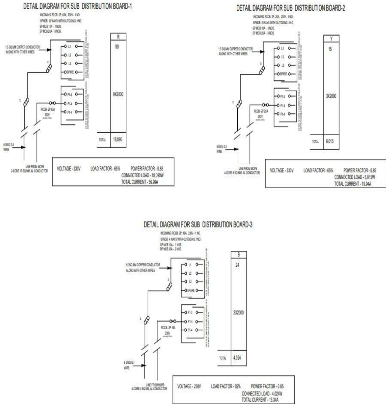
Figure 5.22.7 SDB Detail
