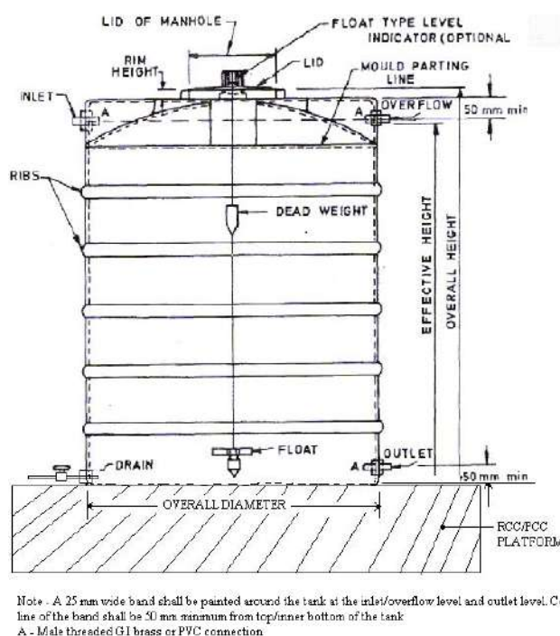
Figure 3.21 TYPICAL DETAILS OF CYLINDRICAL VERTICAL TANK
