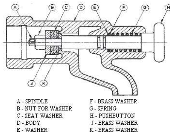
Figure 3.8 SELF-CLOSING TAPS (CONCUSSIVE PUSHBUTTON TYPE - For Heads not exceeding 2 m)
