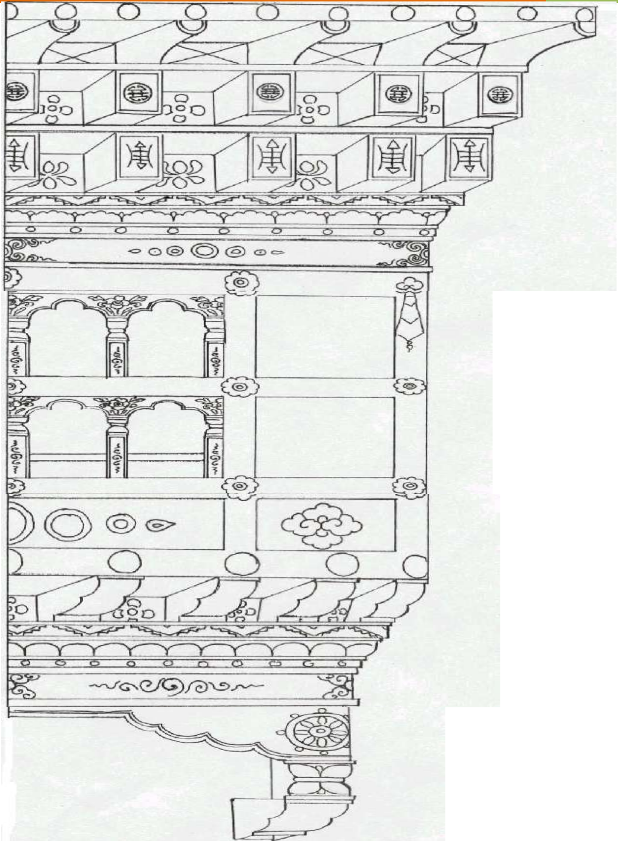
Figure 5.19.5 Rabsey (Thama)
