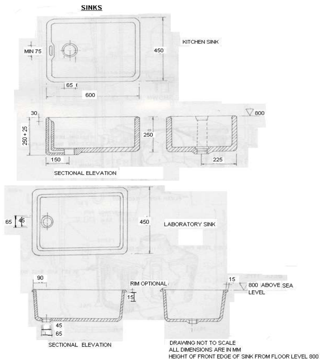
Figure 5.16.4 Kitchen sink
