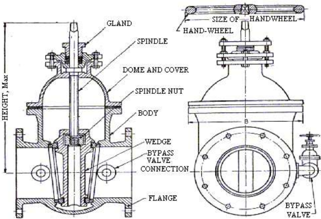
Figure 3.6 TYPICAL SKETCH OF A SLUICE VALVE
