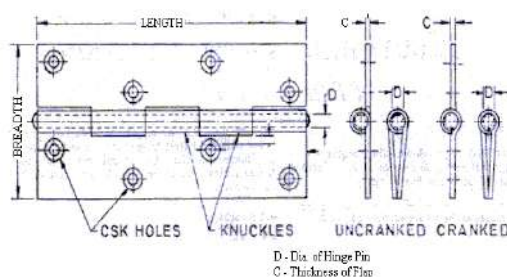
Figure 3.2 A TYPICAL MILD STEEL BUTT HINGE
