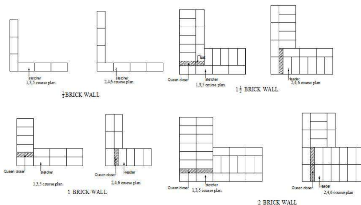
Figure 5.9.1: English Bond
