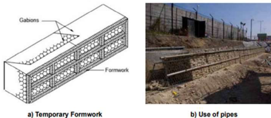
Figure 7 Use of steel frame or pipes to avoid gabion bulging during filling operation
