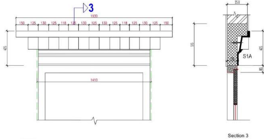
Fig 5.11.3 GRC Door Cornice 1200mm dhung length
