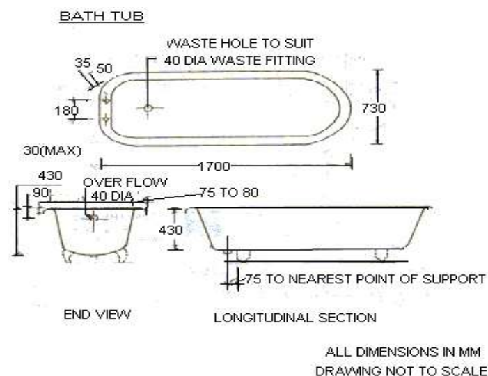
Figure 5.16.2 Details of a bathtub
