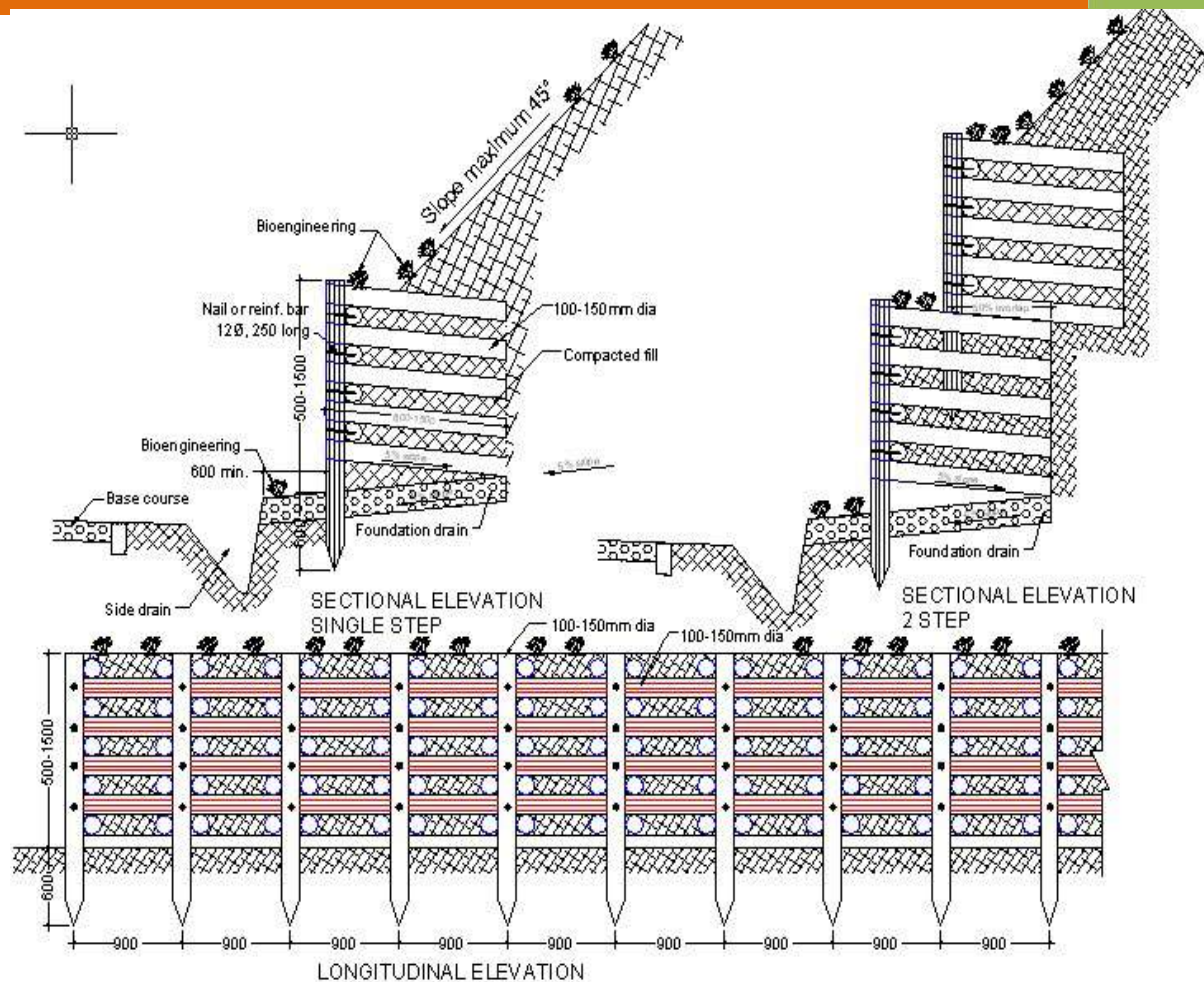
Figure 5.21.3 Crib wall
