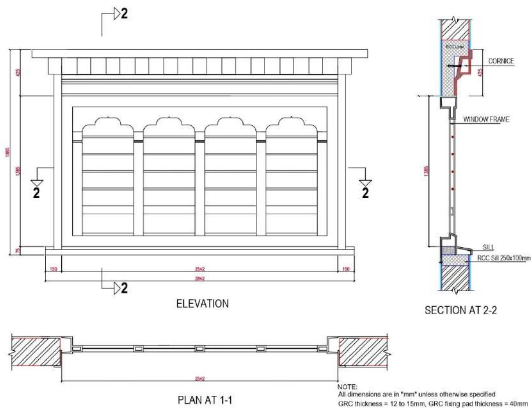
Fig 5.11.13 GRC Window 4 Bay 2542mmX1385mm (Full set)
