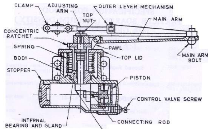
Figure 3.3 Typical Sketch of Hydraulic door closer showing main components (Bottle Type)
