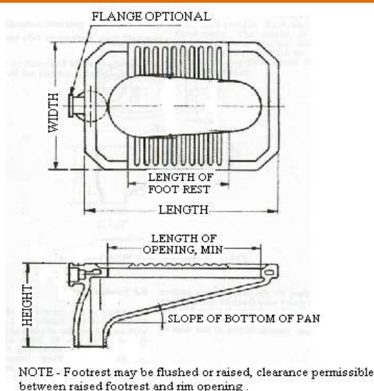
Figure 3.16 ORRISA PATTERN SQUATTING PAN
