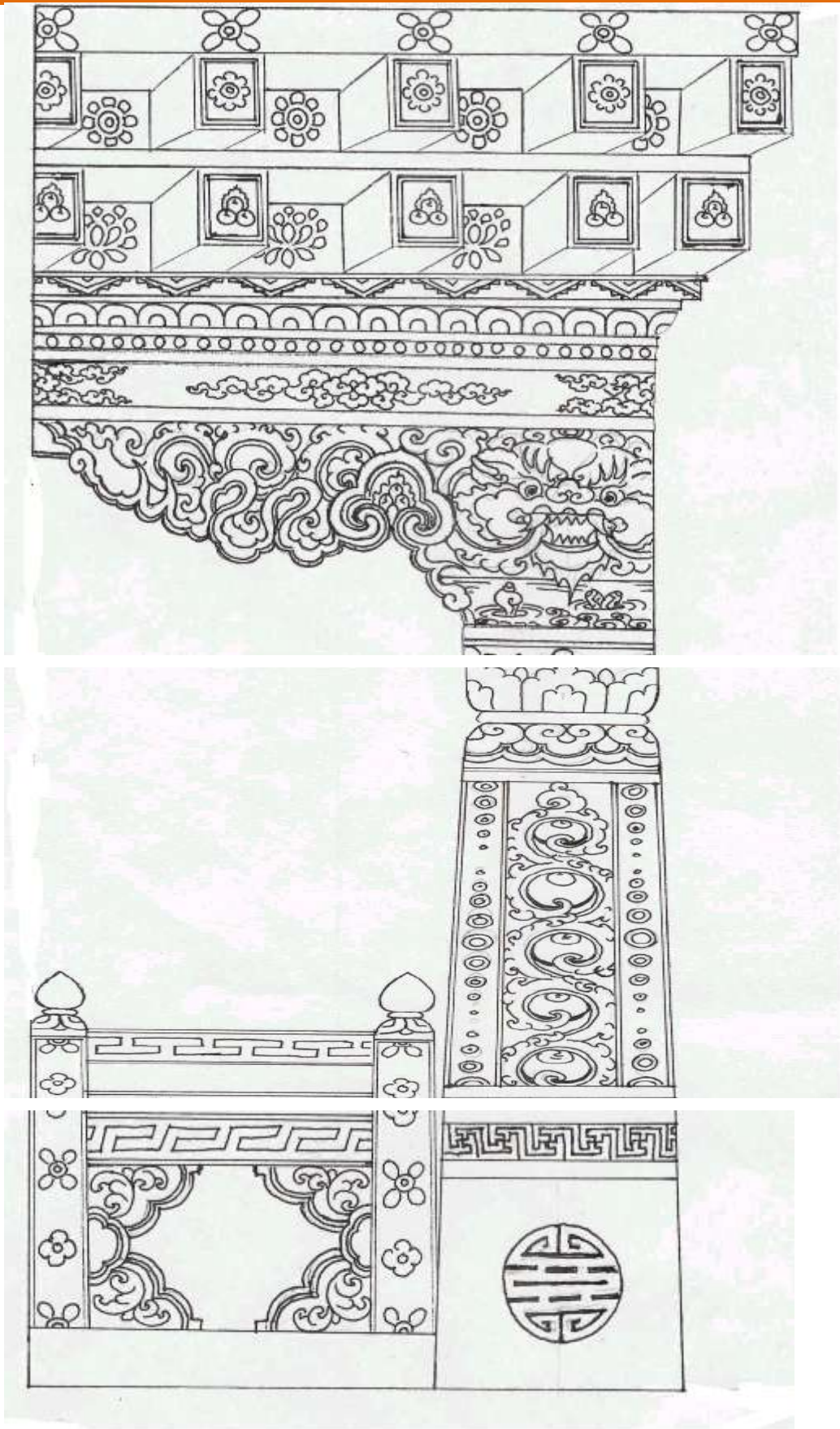
Figure 5.19.11 Kachen (Ding)
