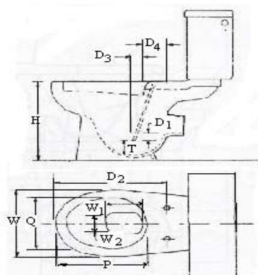
c. WASHDOWN WATER CLOSET FOR CLOSE COUPLED SUITE - CONCEALED S TRAP
