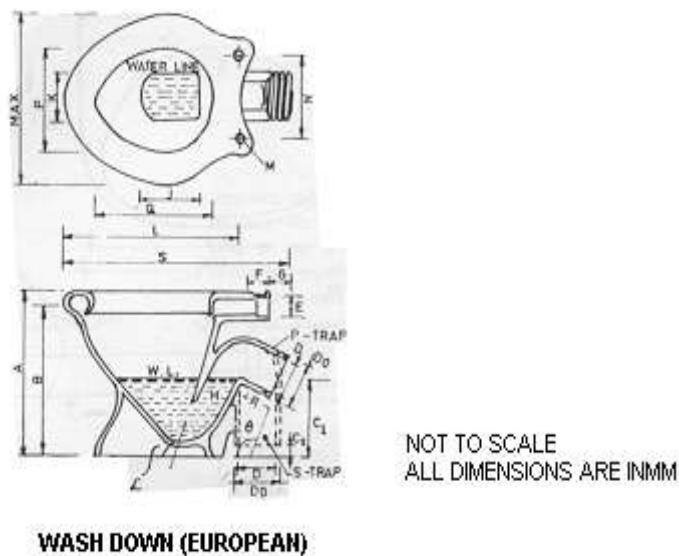
Figure 5.16.1 Water closet
