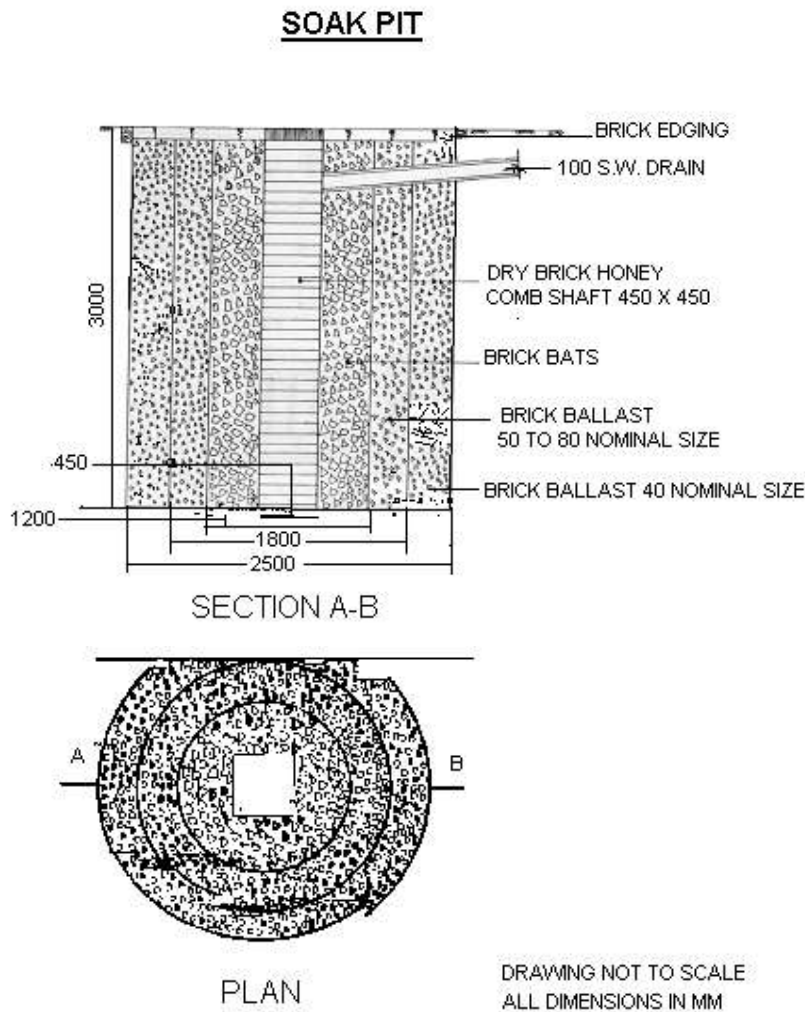
Figure 5.17.4 Soak pit
