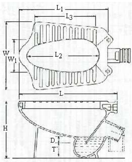
Figure 3.13 UNIVERSAL WATER CLOSET (Functional dimensions)
