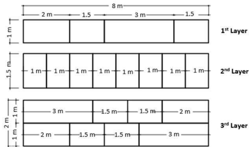
Figure 5.21.2 Retaining wall
