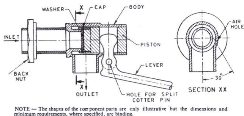
Figure 3.7 BALL VALVE (ASSEMBLY)
