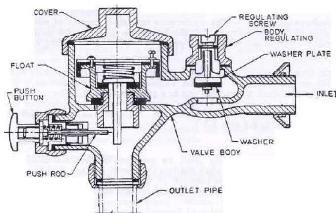
Figure 3.19 TYPICAL SKETCH OF A FLUSH VALVE
