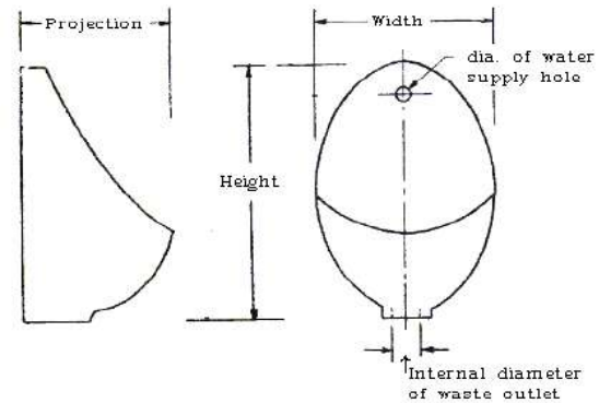
Figure 3.17 (b) BOWL TYPE ANGLE BACK URINAL WITHOUT RIM
