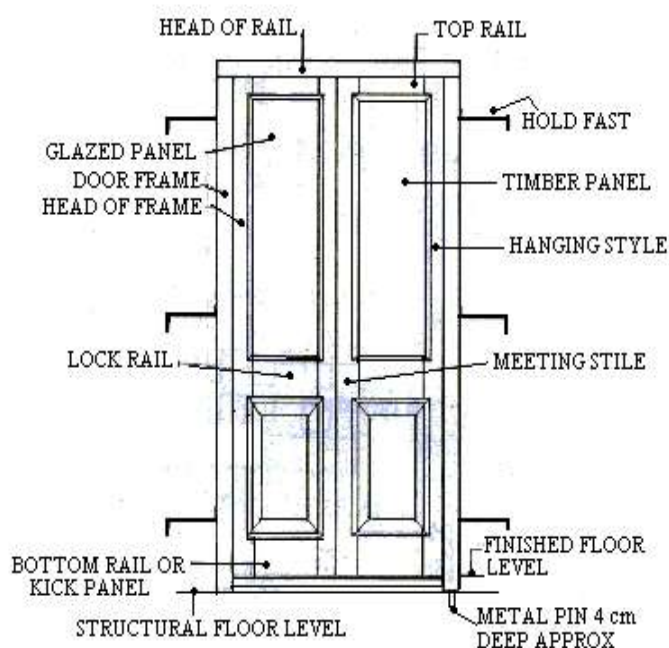
Figure 3.5 TYPICAL ILLUSTRATION OF DOUBLE PANELLED DOOR WITH TIMBER AND GLAZED PANELS
