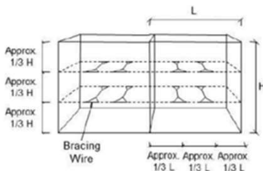
Figure 5 Bracing wire details for 1 m deep gabion crates
