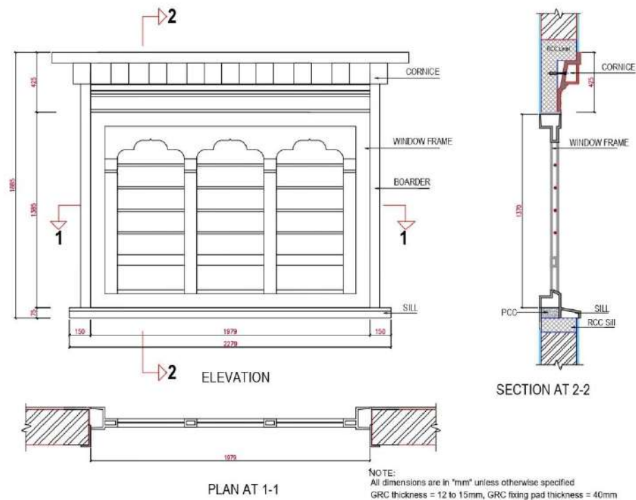
Fig 5.11.12 GRC Window 3 Bay 1416mmX1385mm (Full set)
