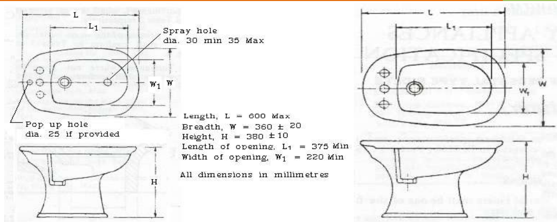
Pattern 1 – Pedestal bidets with flushing rim and spray holes (see fig 3.18 a)
