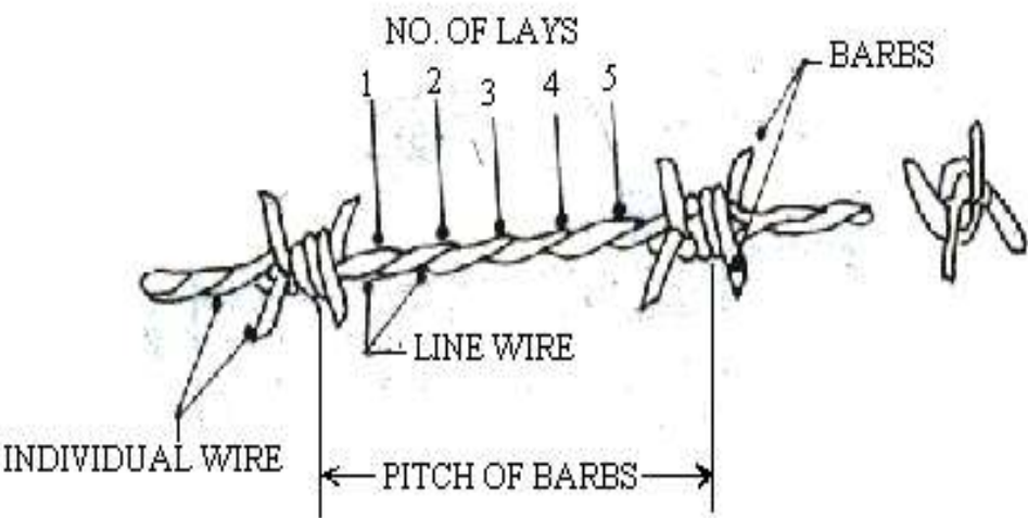
Figure 3.4 DETAILS OF BARBED WIRE (TYPE A)
