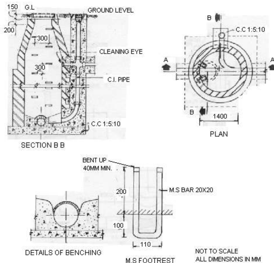
Figure 5.4.4: Drop Manhole
