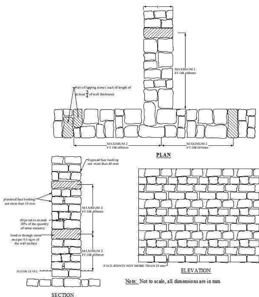
Figure 5.10.1 Random Rubble Masonry
