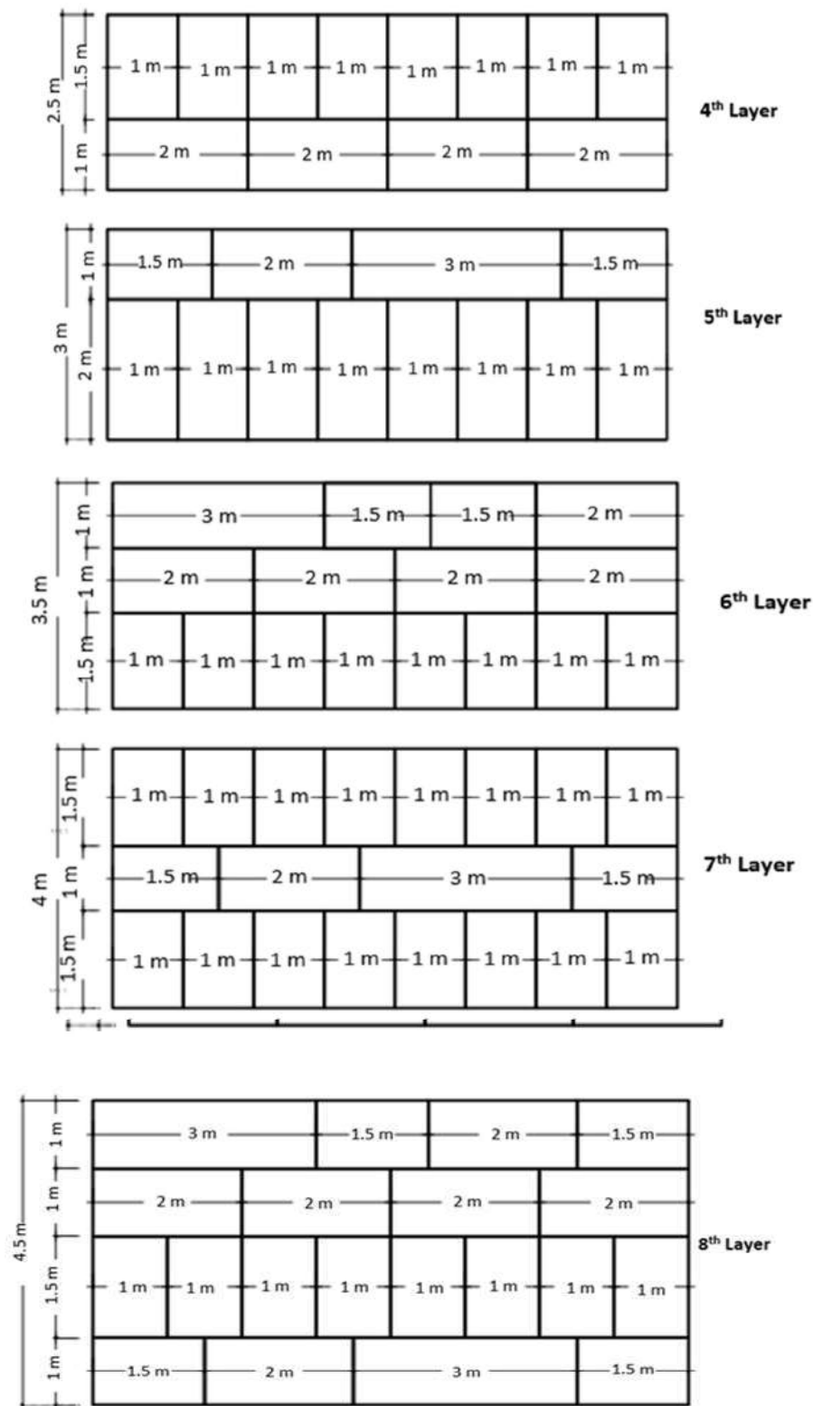
Figure 5.21.3 Wall Plan
