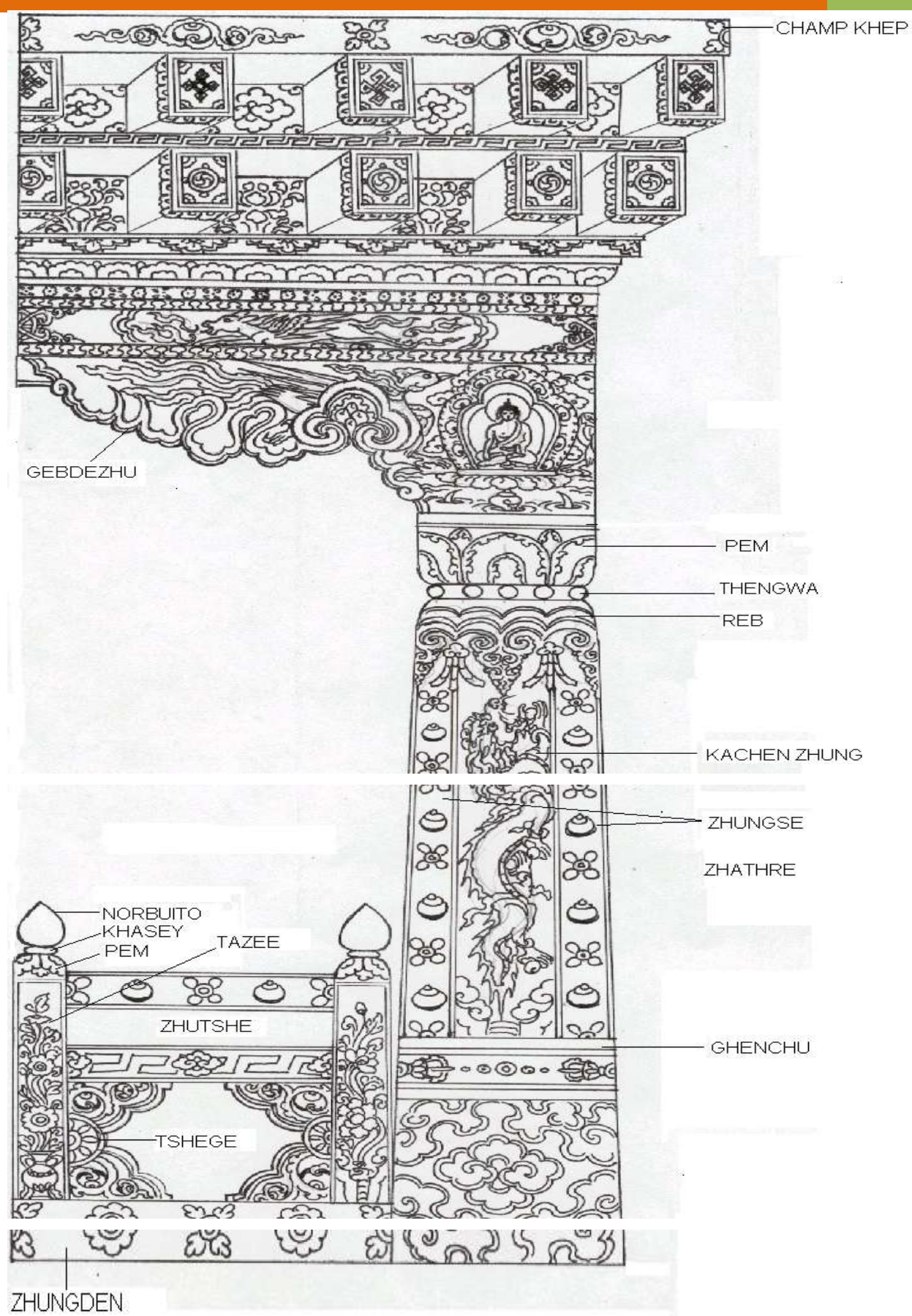
Figure 5.19.10 Kachen (RAB)
