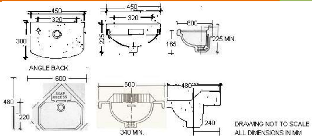
Figure 5.16.3 Types of wash basin
