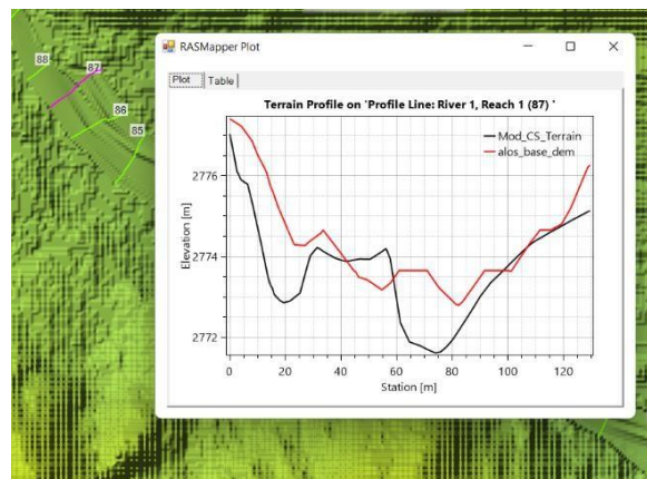
Figure 27: Profile difference in the ALOS DEM and the modified terrain at C/S 87
