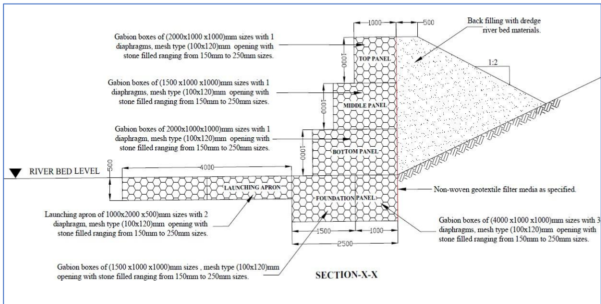
Figure 67: Gabion Wall
