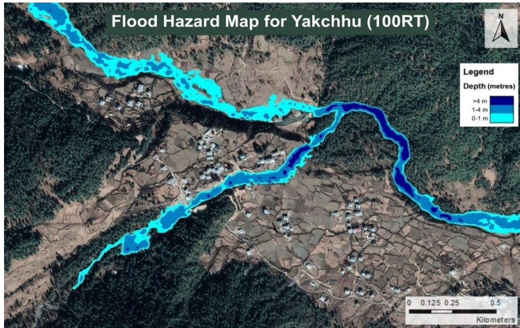
Figure 31: Flood Depth Map for Yakchu Stream
