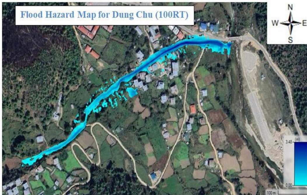
Figure 38: Flood Depth Map for Dung Chu Stream
