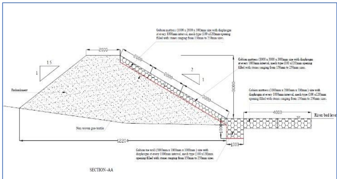
Figure 69: Gabion Revetment
