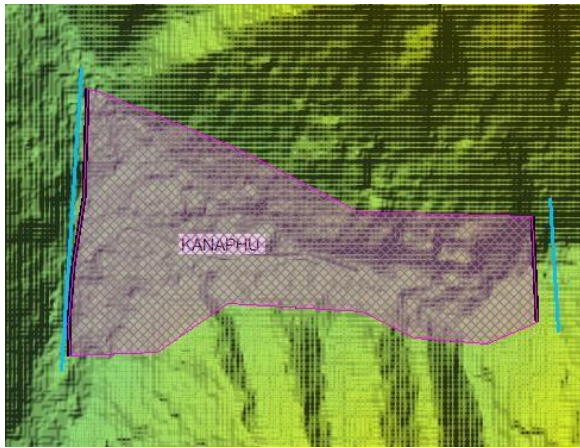
2D flow area for Kanaphuchhu stream
