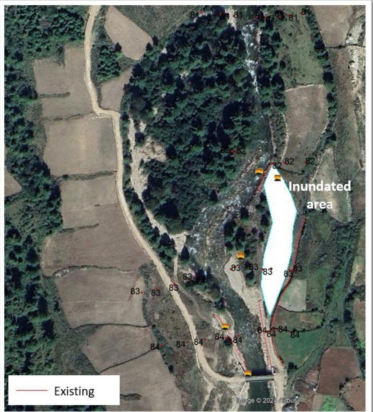
Figure 54: Above the NRDCL depot, the inundation area
