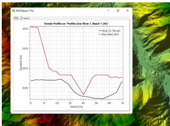
Figure 26: Profile difference in the ALOS DEM and the modified terrain at C/S 34
