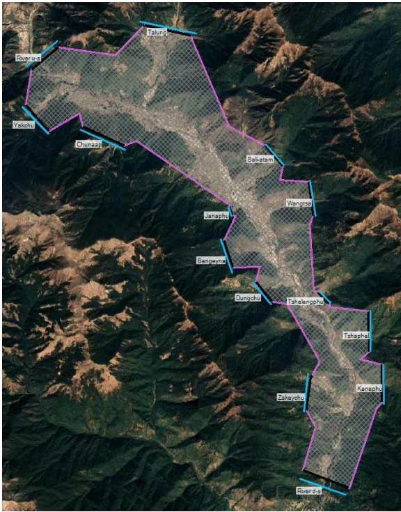
Figure 23: 2D Flow Area of Haachu and Tributaries
